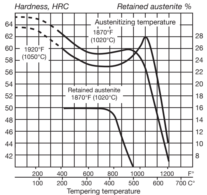
TEMPERING GRAPH
