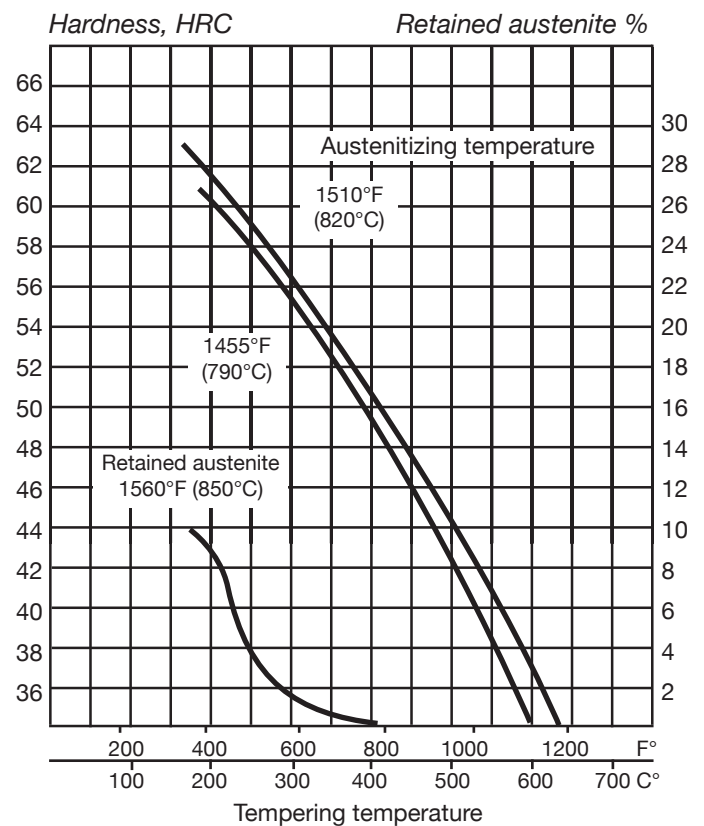
TEMPERING GRAPH
